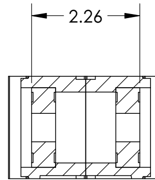
SECTION A-A BEARING SPACING
