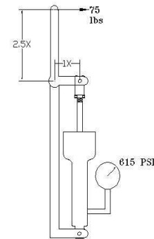
FIG 1 MECH ADV = 2.5/1 = 2.5 to 1
