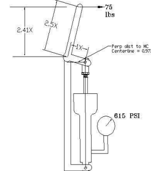
FIG 2 MECH ADV = 2.41/0.96 = 2.5 to 1
