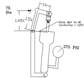
FIG 2 MECH ADV = 1.45/1.29 = 1.12 TO 1
