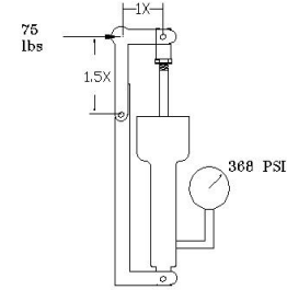
FIG 1 MECH ADV = 1.5/1 = 1.5 to 1
